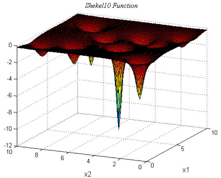
Fig.1. Shekel10 function.
